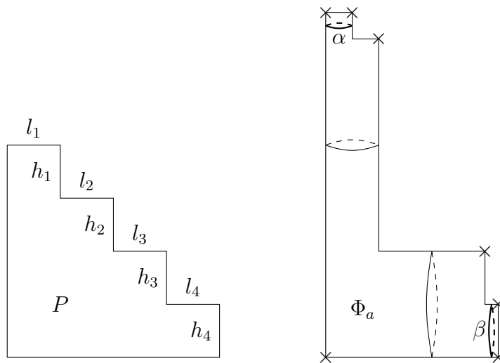
Figure 1. The staircase-shaped polygon P and the half-translation surface \Phi_a .
