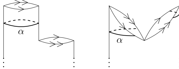
Figure 3. Left: adding a handle to \Phi_a . Right: another representation of \Phi_a obtained by cut-and-paste.
